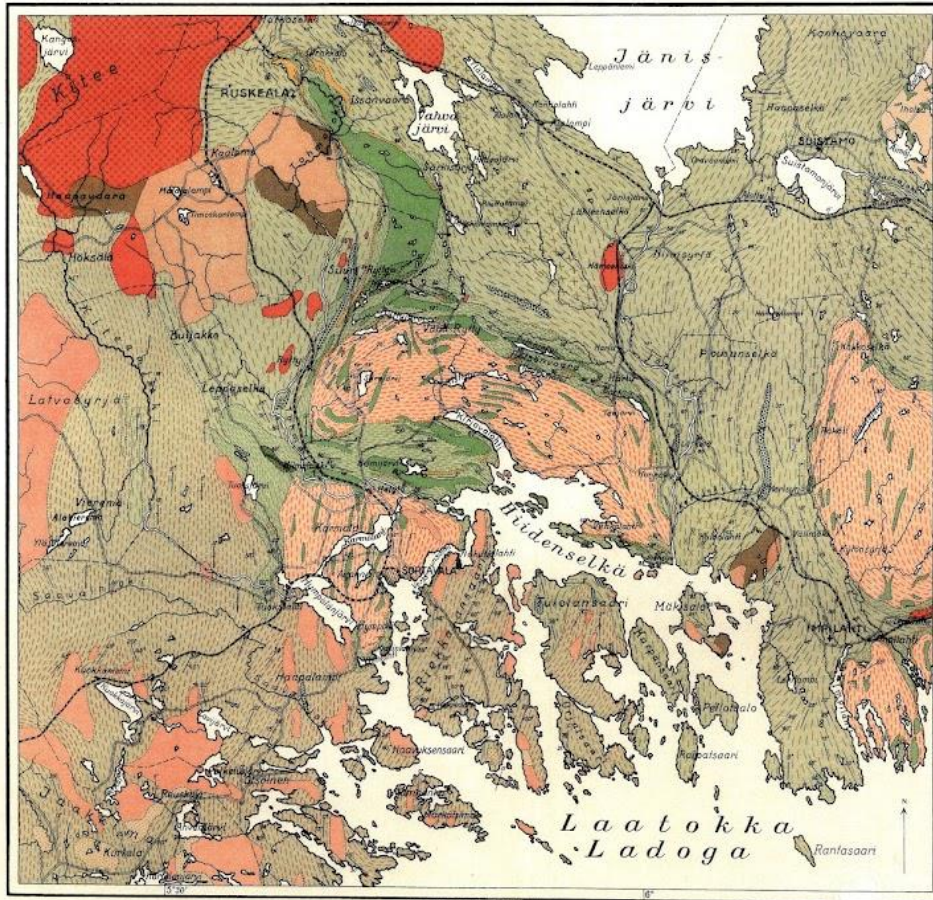
geological map of the area
