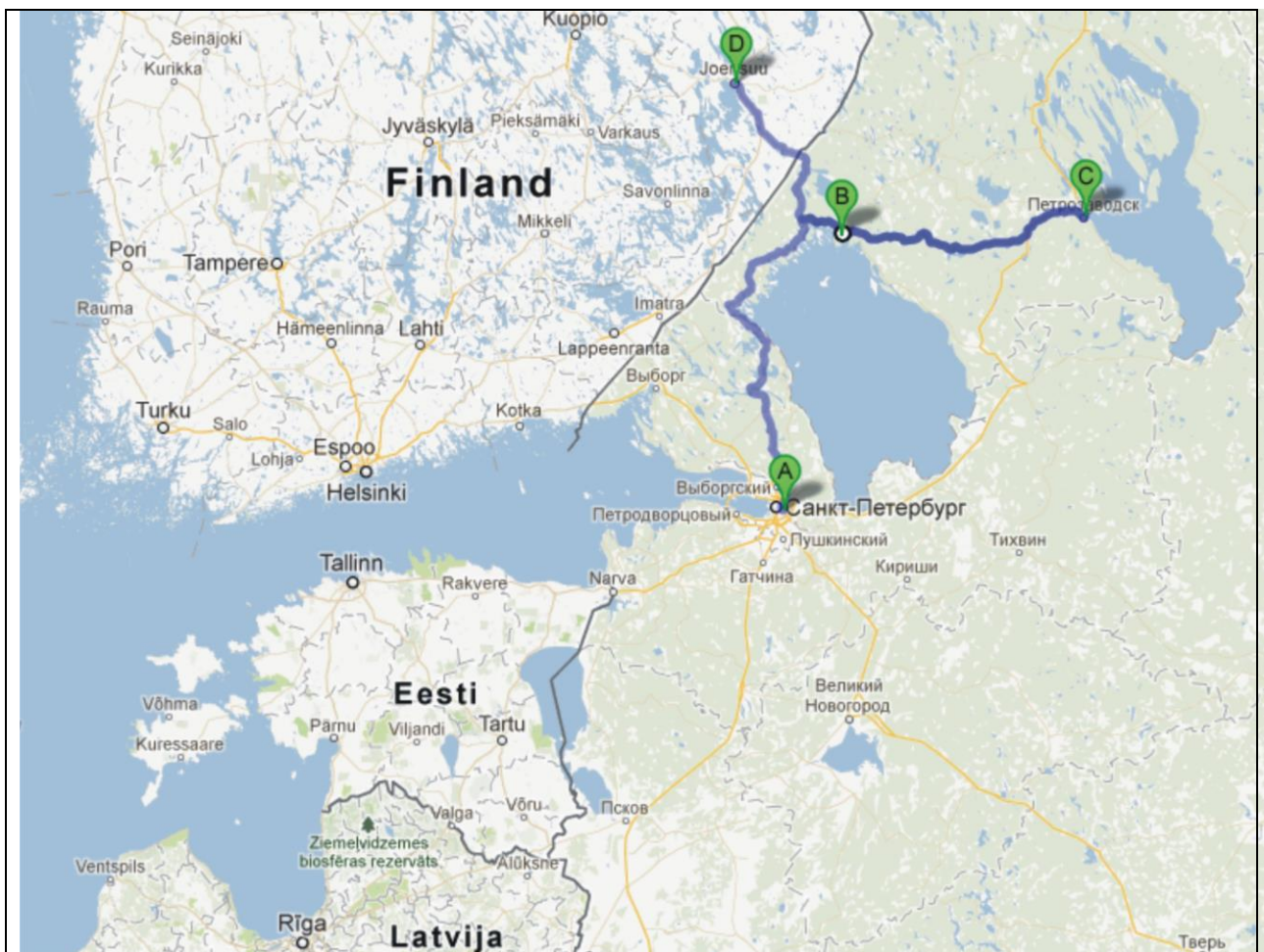
Location map: A – City of St.Petersburg; B – Impilahti village; C – Petrozavodsk; D – Joensuu.
